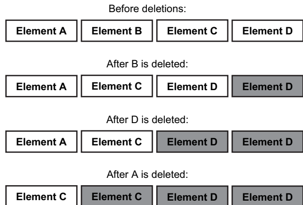
Fig. 7 – Hypothetical subkey deletion sequence.
