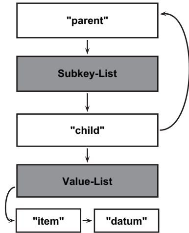
Fig. 6 – Simple example: physical view.
