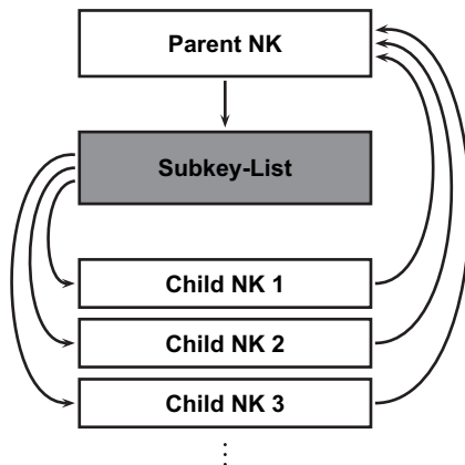
Fig. 3 – Key-related pointers.
