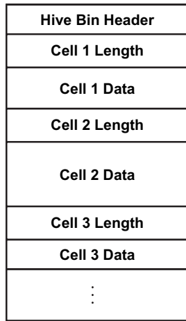
Fig. 2 – Hive bin structure.
