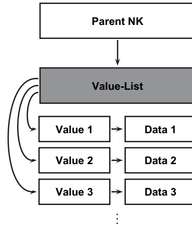
Fig. 4 – Value-related pointers.
