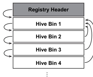
Fig. 1 – Top-level registry structure.
