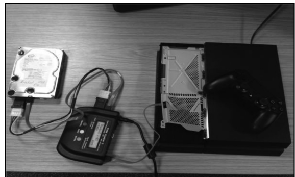
Fig. 4. A PlayStation 4 hard drive connected via the Voom Shadow 3.
