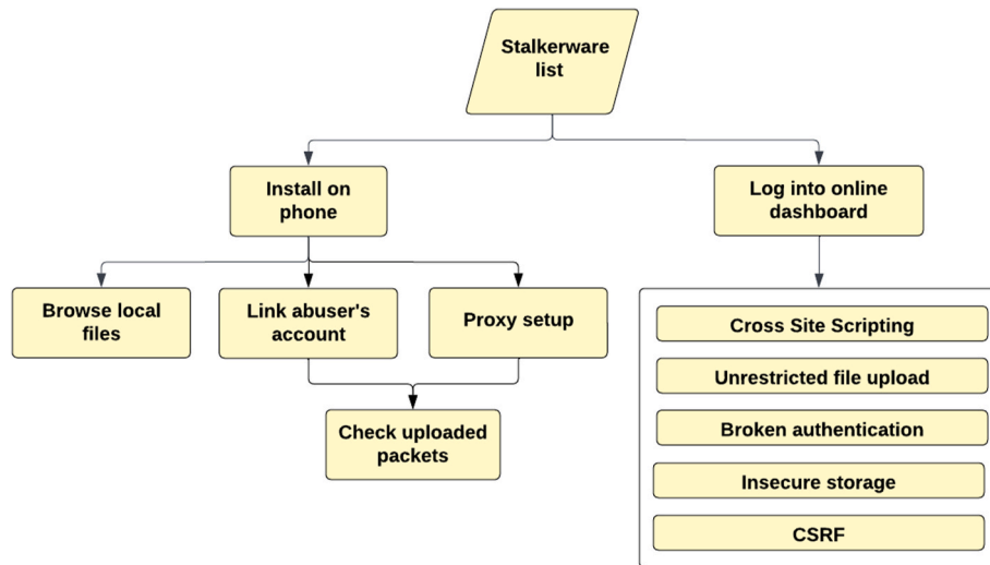
Fig. 2. Overview of the stalkerware security analysis methodology.
