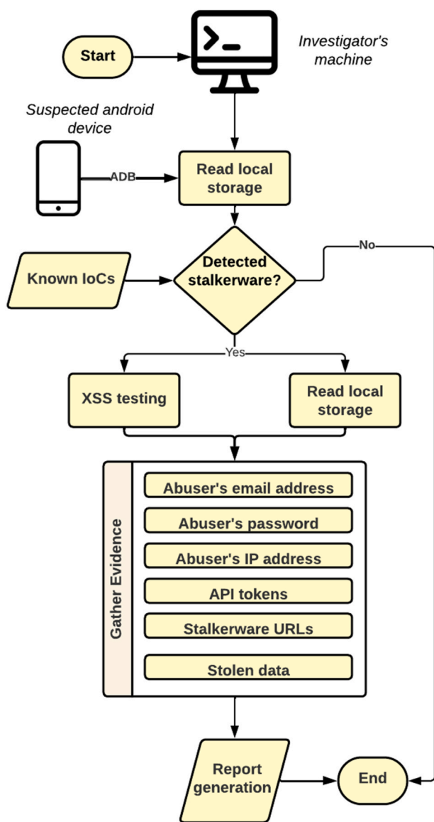
Fig. 3. WARNE's evidence collection process.
