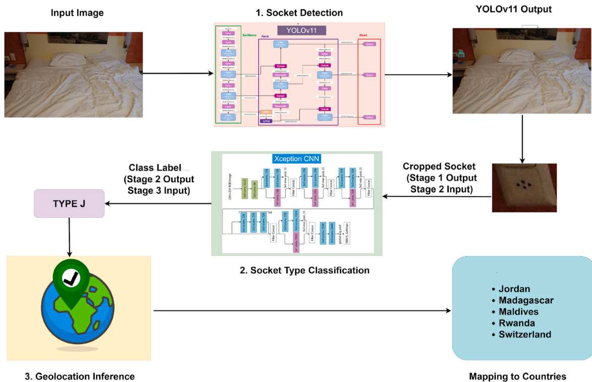
Fig. 2. Architecture of the proposed three-stage pipeline: (1) Socket detection, (2) Socket type classification, and (3) Geolocation.
