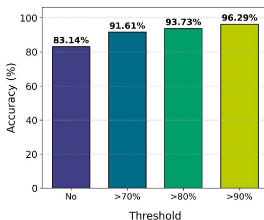
Fig. 6. Country prediction accuracy by varying socket type confidence threshold values.
