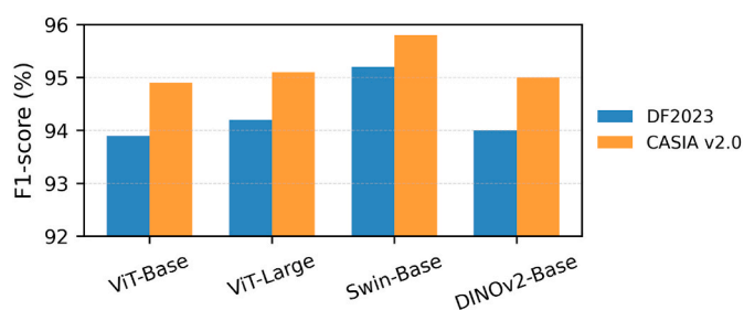
Fig. 4. F_x backbone component analysis showing F1-scores on DF2023 and CASIA v2.0. ViT-Base offers the best balance between accuracy and efficiency.
